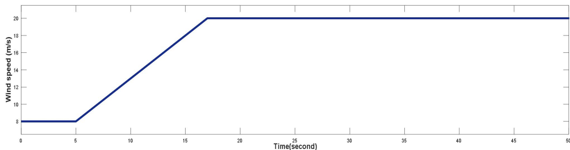
Figure 19. Wind speed changes 8–20m/s.
