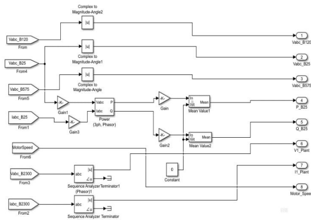
Figure 8. Acquisition of data from grid.
