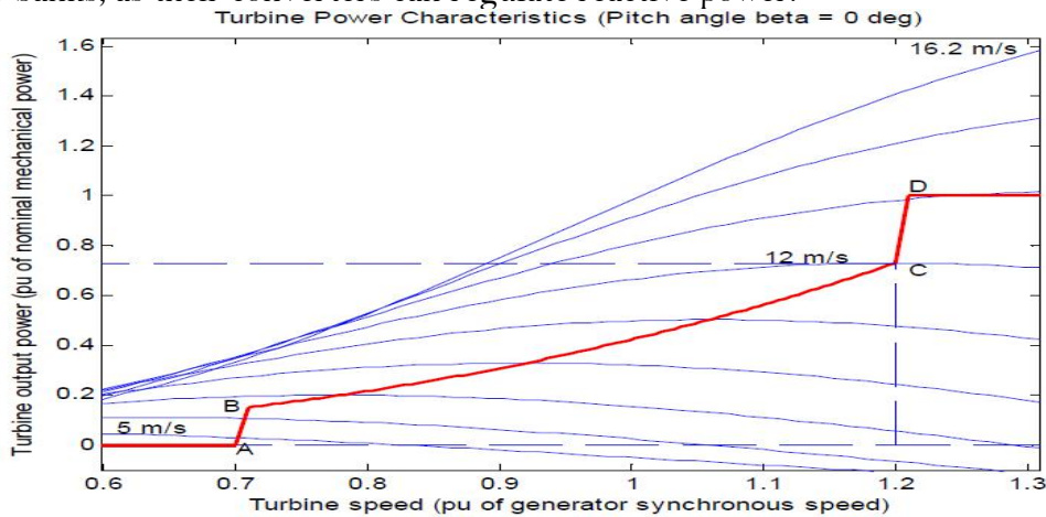
Figure 4. Turbine power characteristics
