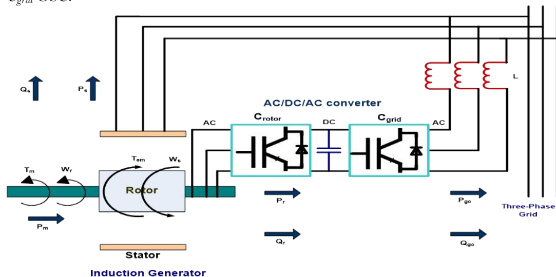
Figure Error! No text of specified style in document.. Power flow diagram of DFIG.
