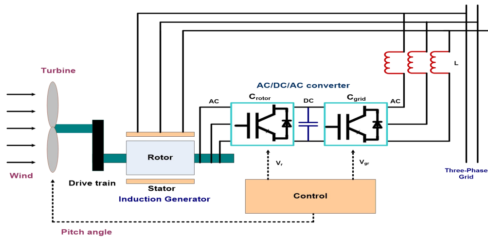
Figure 2. Wind turbine configuration with variable speed and DFIG.
