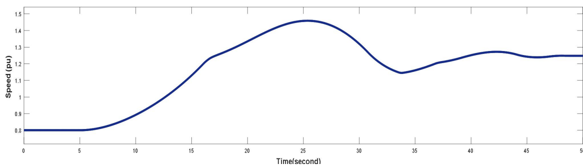
Figure 20. Turbine rotor speed when speed changes 8-20 m/s.
