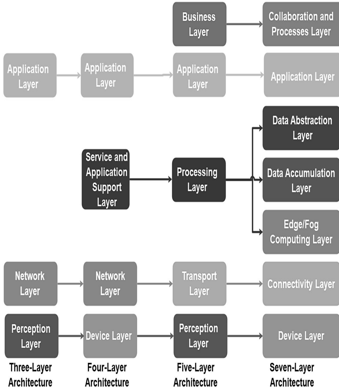
FIGURE 2: LAYERS OF IIOTS FOR SECURE NETWORK [20]
