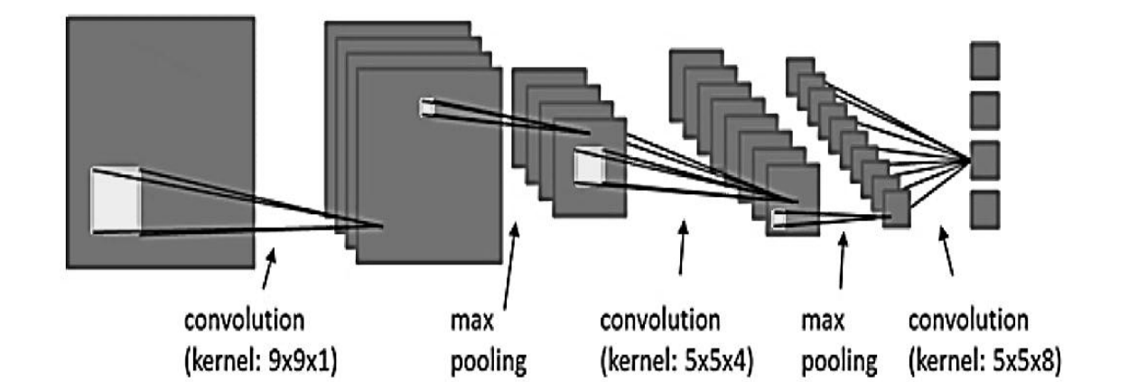
FIGURE 8: PROPOSED MACHINE LEARNING BASED CNN ARCHITECTURE FOR IIOTS
