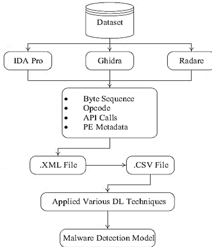
FIGURE 7: FLOW CHART FOR MACHINE LEARNING BASED STATIC INTRUSION DETECTION FOR IIOTS
