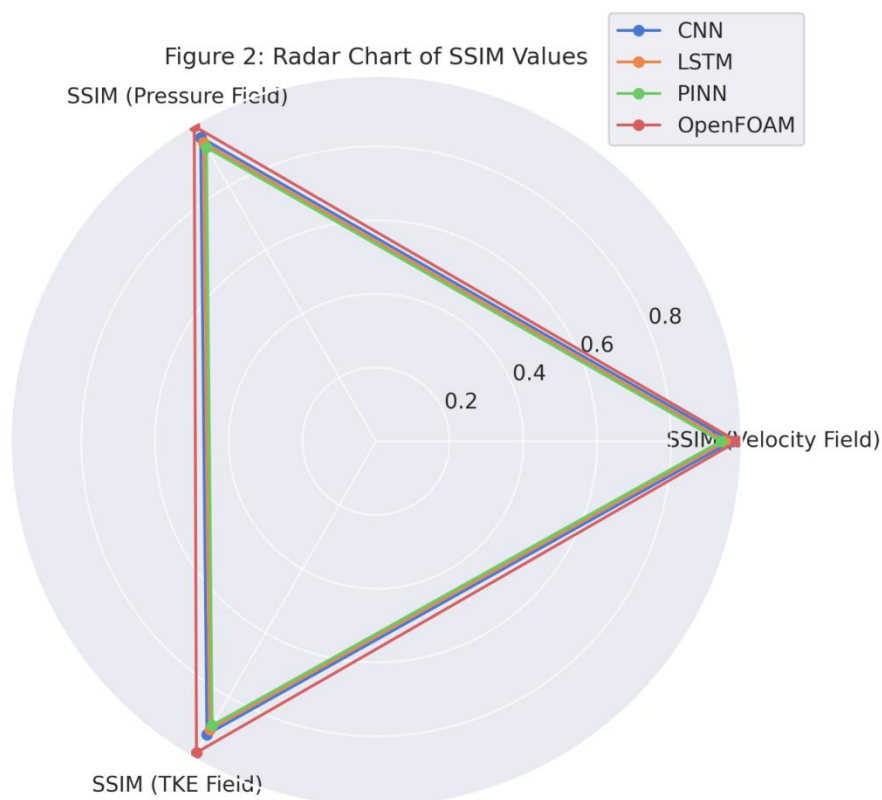
Figure 2: Structural Similarity Index (SSIM) comparisons across velocity, pressure, and turbulence fields.
