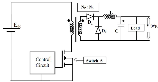
FIG 6; FORWARD CONVERTER
