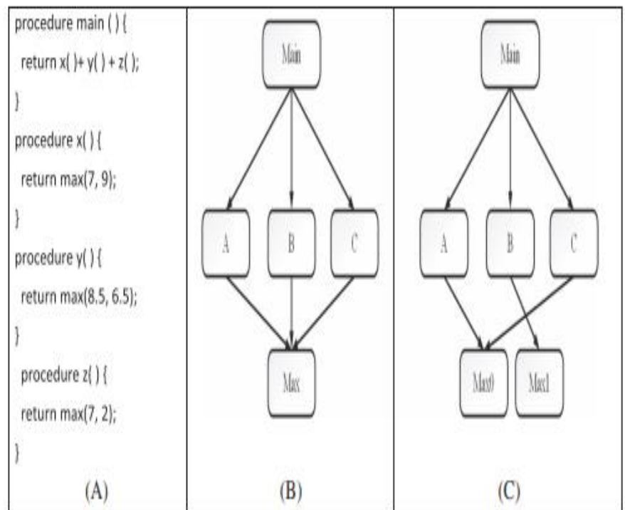
FIGURE 2 Call graphs for permission analysis ((A) example program, (B) context-insensitive, and (C) context-sensitive) 21
