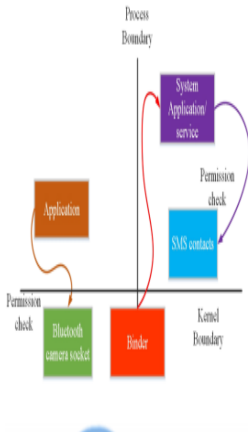
FIGURE 3 Permission enforcement in Android application
