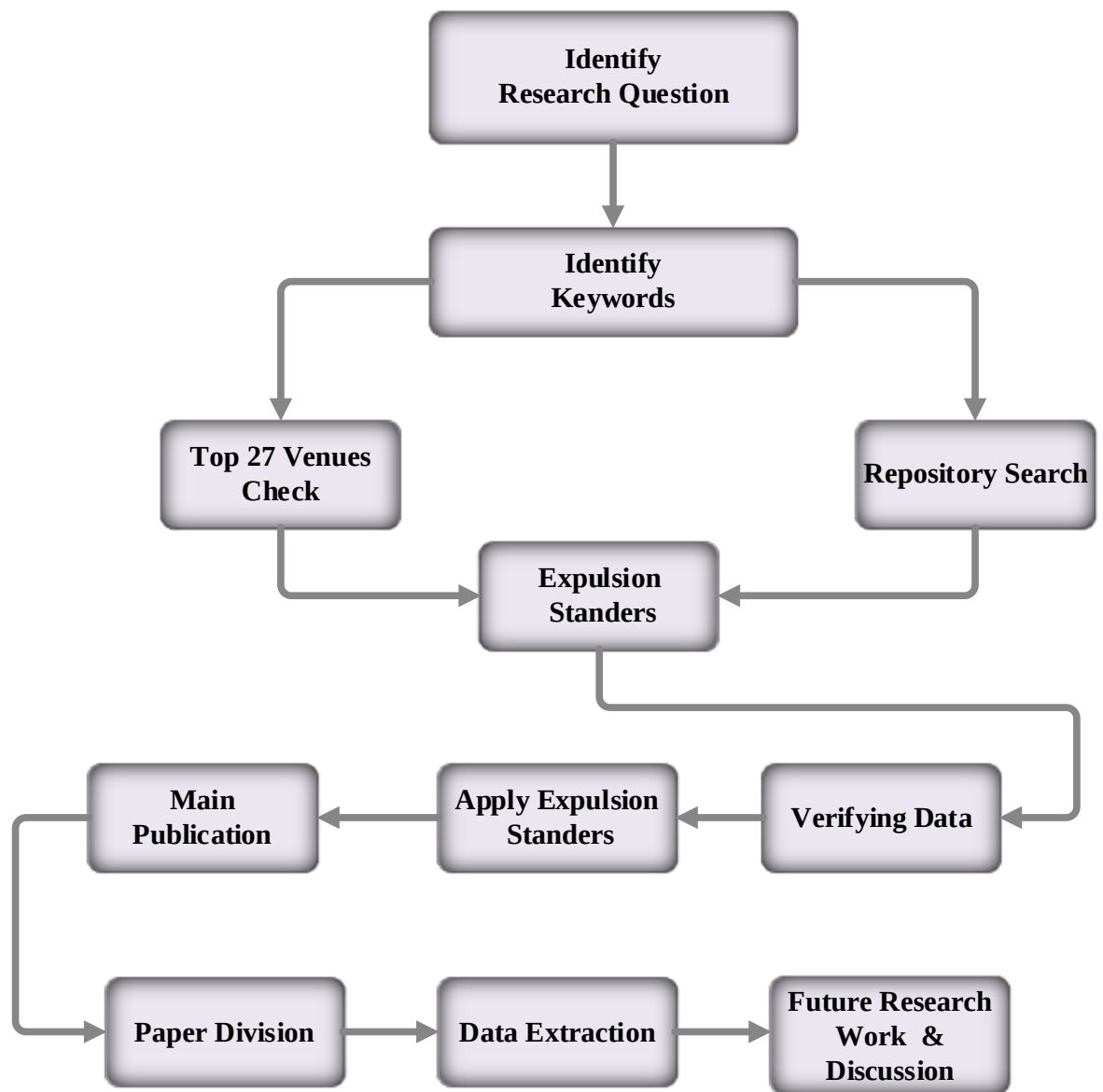
FIGURE 5 Methodologies
